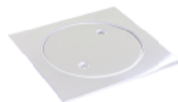
Clean Out Floor Drain with Removable Cover and Securing Screws Stainless Steel Grade 304 Vertical Outlet Dia. 134 mm 200 x 200 mm
